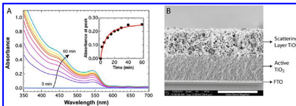
Figure 3. (A) Absorption spectra of a red QD attached to a transparent \text{TiO}_2 by EPD with a bias voltage of 60 V at different times from 0 to 60 min. The data were collected at 0, 2, 5, 10, 15, 20, 25, 30, 40, and 60 min. The inset shows the variation of the absorption peak intensity at 550 nm with time. (B) Cross-sectional SEM image of the photoanode consisting of a \text{TiO}_2 mesoscopic film loaded with QDs. The scale bar represents a length of 10 \mu\text{m} . (Reproduced from ref 25.)
