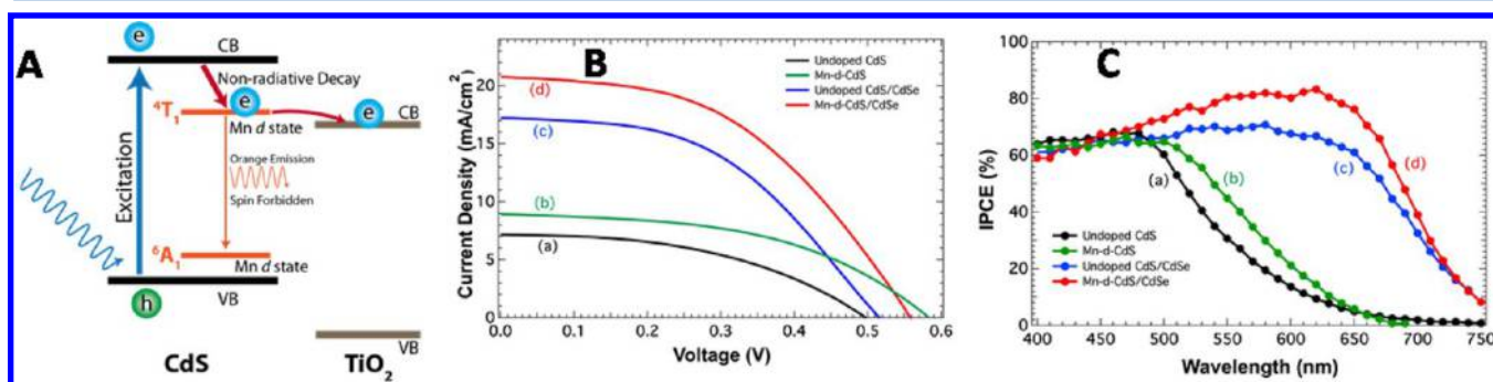
Figure 6. (A) Schematic representation of the energy diagram of Mn-doped CdS. The electron from the conduction band of CdS transfers to the Mn d state ( ^4T_1 ) within a few picoseconds, but the Mn d–d transition has a lifetime in the range of several hundreds of microseconds due to the spin and orbitally forbidden transition. 39 (B) J – V characteristics and (C) Incident photon to charge carrier generation efficiency (IPCE) response of different working electrodes measured under simulated AM 1.5 sunlight ( 100 \text{ mW/cm}^2 ). (a) Undoped CdS, (b) Mn-doped CdS, (c) undoped CdS/CdSe, and (d) Mn-doped CdS/CdSe. The working electrode areas were 0.20, 0.20, 0.22, and 0.22 \text{cm}^2 , respectively (with a \text{Cu}_2\text{S} /RGO counter electrode and aqueous 1 \text{ M S}^{2-}/1 \text{ M S} as the electrolyte). (Reproduced from ref 40.)
