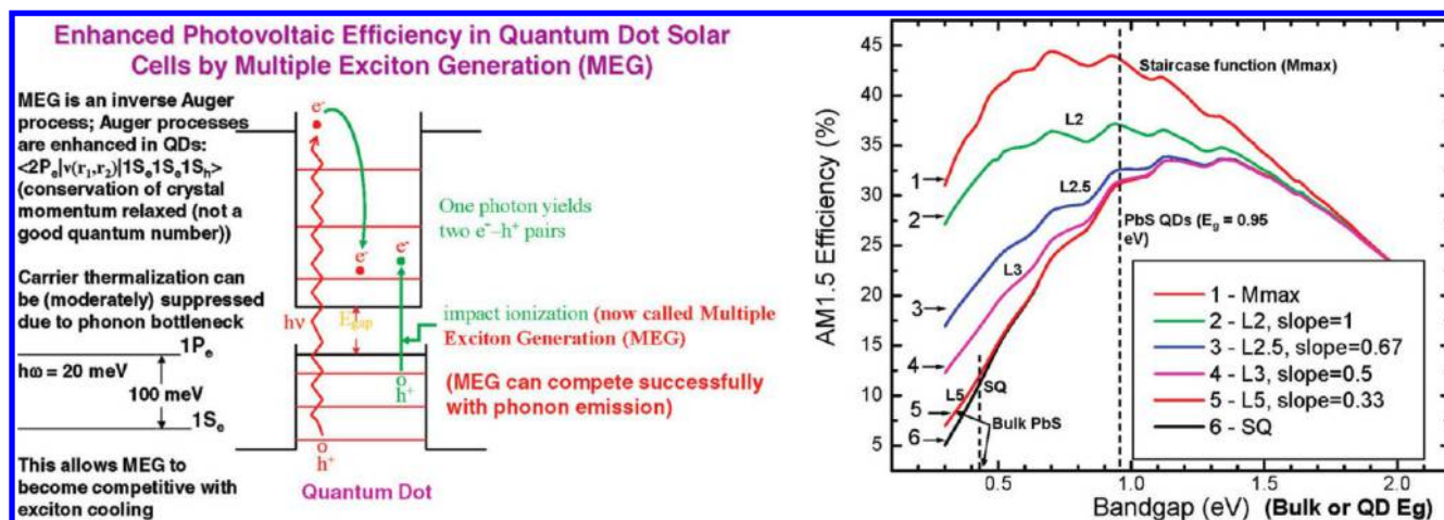
Figure 8. (Left panel) Schematic diagram illustrating the principle of MEG (multiple exciton generation) in QDs. (Right panel) Shockley and Queisser Limit calculations for PV power conversion efficiency for various MEG characteristics in QD solar cells compared to PV cells based on bulk semiconductors. L(n) represents the MEG photon energy threshold in units of the number of band gaps of energy, and the slope value is the MEG efficiency (extra excitons/band gap of the photon energy) beyond the MEG threshold. (Reproduced from ref 57.)
