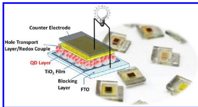
Figure 4. Anatomy of QDSC depicting different layers. The hole transport layer is a redox electrolyte in liquid junction solar cells and a solid-state hole-transporting layer in heterojunction solar cells. The background image shows a few QDSC samples prepared in our laboratory with an active QD layer ( \sim 0.25 \text{ cm}^2 area) sandwiched between the two OTE and the redox electrolyte.
