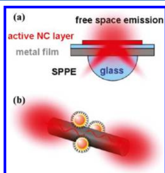
Figure 9. Typical configurations of metal–semiconductor nanostructures that lead to exciton–SP energy transfer. (a) Excited semiconductor NCs that are deposited on a metal film release their energy into free space emission or excite SPs on the metal surface that then can decay radiatively and generate SP emission (SPPE). A dielectric spacer layer prevents close contact between metal and semiconductor components and avoids NC emission quenching caused by coupling to lossy surface waves. (b) NCs attached to a metal nanorod can excite single SPs that propagate along the metal wire, enabling nanoscale energy transport and localization. Because the propagating SPs rapidly remove the energy from the location of the NCs, energy back transfer is unlikely. (Reproduced from ref 68.)
